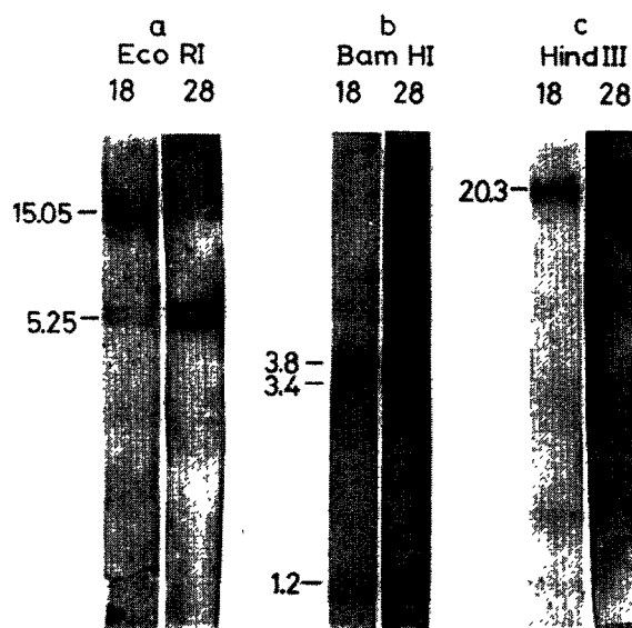
Fig.1. Fluorography of chicken embryo rDNA restriction fragments obtained by cleavage with EcoRI (a), BamHI (b) or HindIII (c) and hybridization with ^{125}\text{I} -labelled 18 S or 28 S rRNA.
